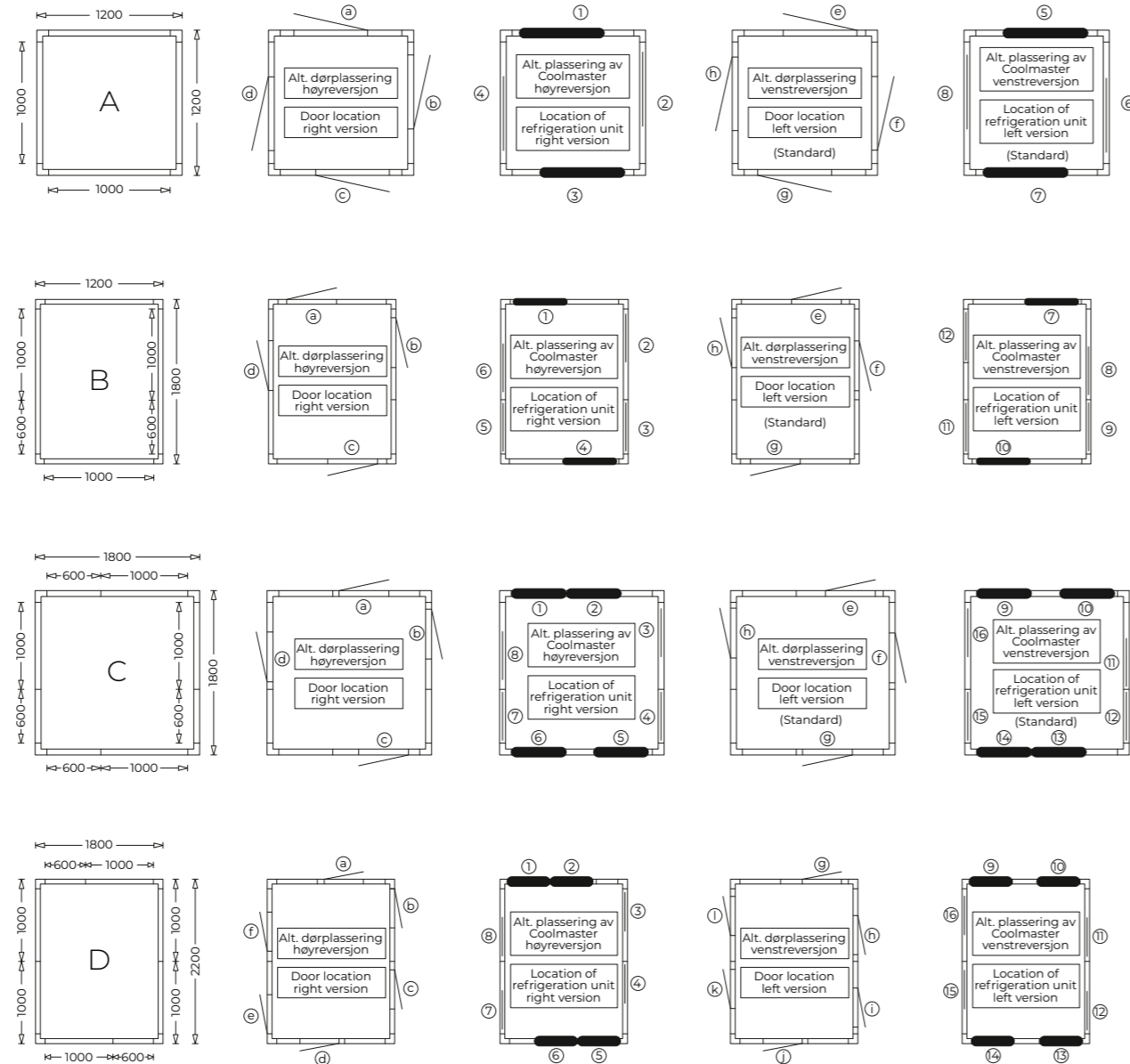
Combination options for placement of door and unit.
